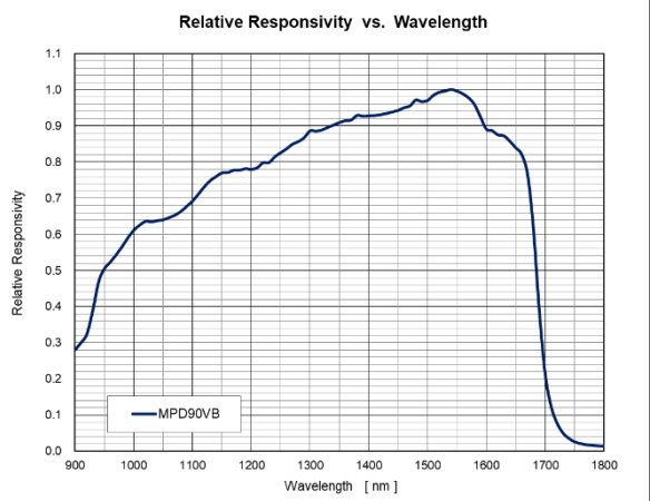
Fig 1. Relative Responsivity vs Wavelength
