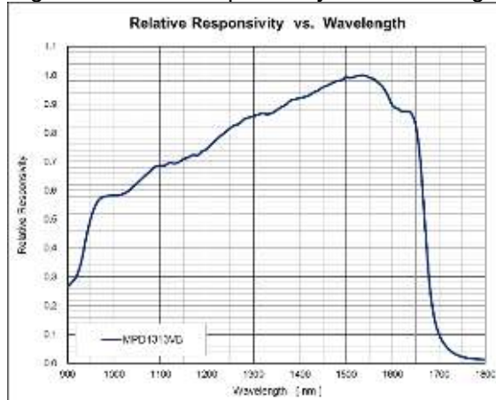
Fig 1. Relative Responsivity vs Wavelength
